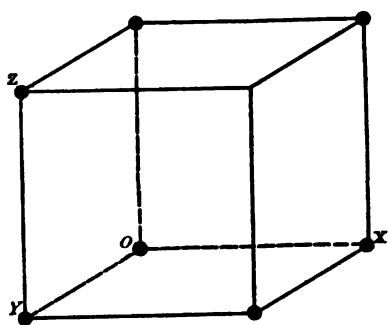
FIG. 28. If OX \neq OY \neq OZ and ZY is normal to the plane YOX but \angle YOX \neq 90^\circ , this is the unit of \Gamma_m ; if the three edges are mutually perpendicular and (1) OX \neq OY \neq OZ , the unit corresponds to \Gamma_o , (2) if OX = OY \neq OZ it corresponds to \Gamma_1(a) or (3) if OX = OY = OZ the unit is that of \Gamma_c .
